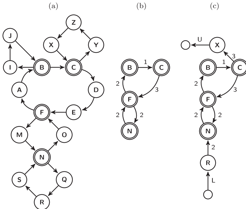
Fig. 4. A graph representation of the voyage edges in a small instance with five rotations. All edges have a cost of one. There are four minor hubs B , C , F and N , where transshipments from one rotation to another are possible. Load, unload and transshipment edges have been excluded for simplicity.
