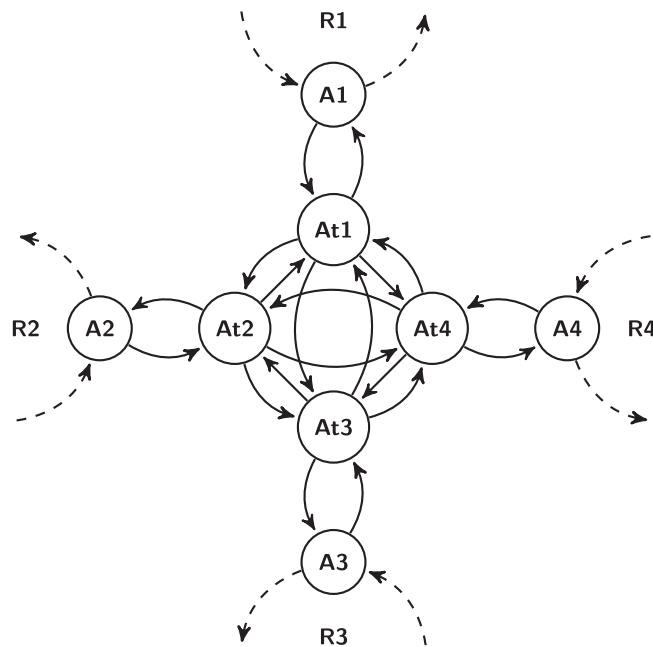
Fig. 11. A general transshipment structure shown for a physical port, A , with four rotations visiting the port. A1 , A2 , A3 , and A4 are the corresponding port calls. At1 , At2 , At3 , and At4 are extra transshipment nodes and edges are added between all pairs of these. Solid edges correspond to transshipment edges and dashed to voyage edges.
