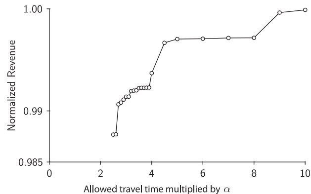
Fig. 15. Sensitivity of limits on travel time in terms of revenue based on the data for an instance of WS (WS0).
