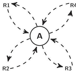
Fig. 6. Simple transshipment structure shown for a physical port, A, with four rotations visiting the port. Voyage edges are dashed and cargo transship directly from one voyage edge to another.
