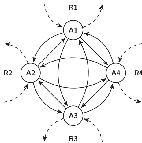
Fig. 8. The complete transshipment structure shown for a physical port, A , with four rotations visiting the port. A1 , A2 , A3 , and A4 are the corresponding port calls. Solid edges correspond to transshipment edges and dashed to voyage edges for the four different rotations visiting port A .
