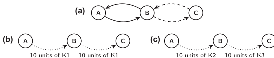
Fig. 2. (a) A simple example network with two rotations R1 (solid edges) and R2 (dashed edges). (b) and (c) Show two possible flows in the network. The paths for commodities K1, K2, and K3 are marked by dotted edges.
