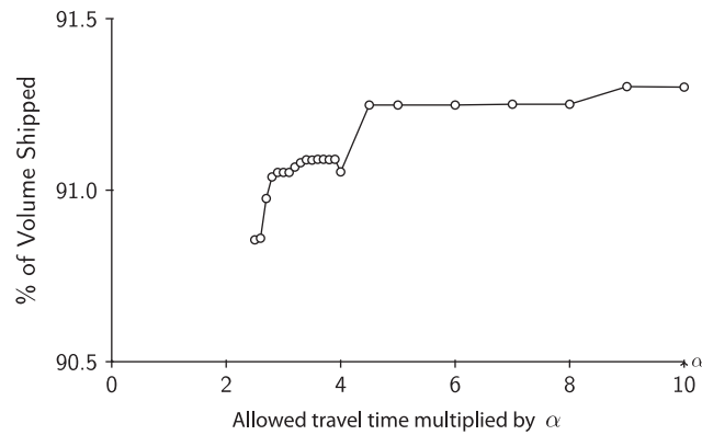
Fig. 13. Sensitivity of limits on travel time in terms of volume shipped based on the data for an instance of WS (WS0).
