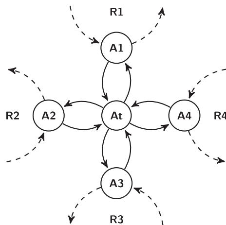
Fig. 9. The star transshipment structure shown for a physical port, A , with four rotations visiting the port. A , A2 , A3 , and A4 are the corresponding port calls and At is an extra transshipment node. Solid edges correspond to transshipment edges and dashed to voyage edges for the four different rotations visiting port A .
