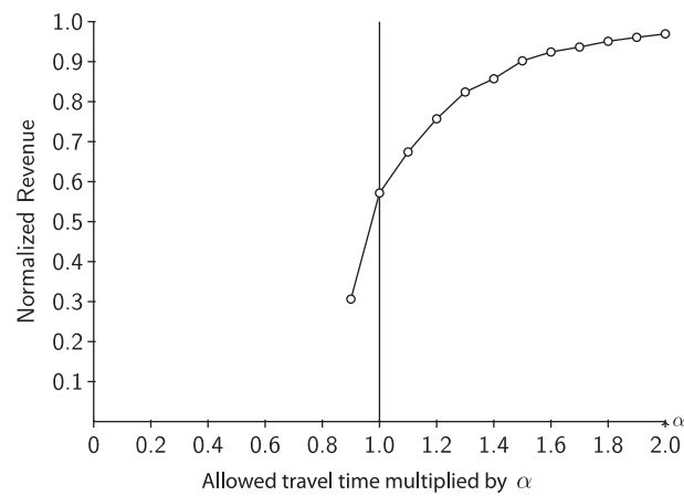
Fig. 14. Sensitivity of limits on travel time in terms of revenue based on the data for an instance of WS (WS0).
