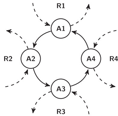
Fig. 7. The transshipment structure shown for a physical port, A , with four rotations visiting the port. A1 , A2 , A3 , and A4 are the corresponding port calls and they are connected in a ring. Solid edges correspond to transshipment edges and dashed to voyage edges.
