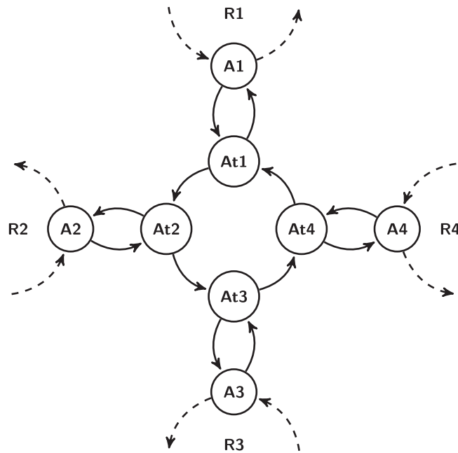
Fig. 10. The ring transshipment structure shown for a physical port, A , with four rotations visiting the port. A1 , A2 , A3 , and A4 are the corresponding port calls. At1 , At2 , At3 , and At4 are extra transshipment nodes. Solid edges correspond to transshipment edges and dashed to voyage edges for the four different rotations visiting port A .
